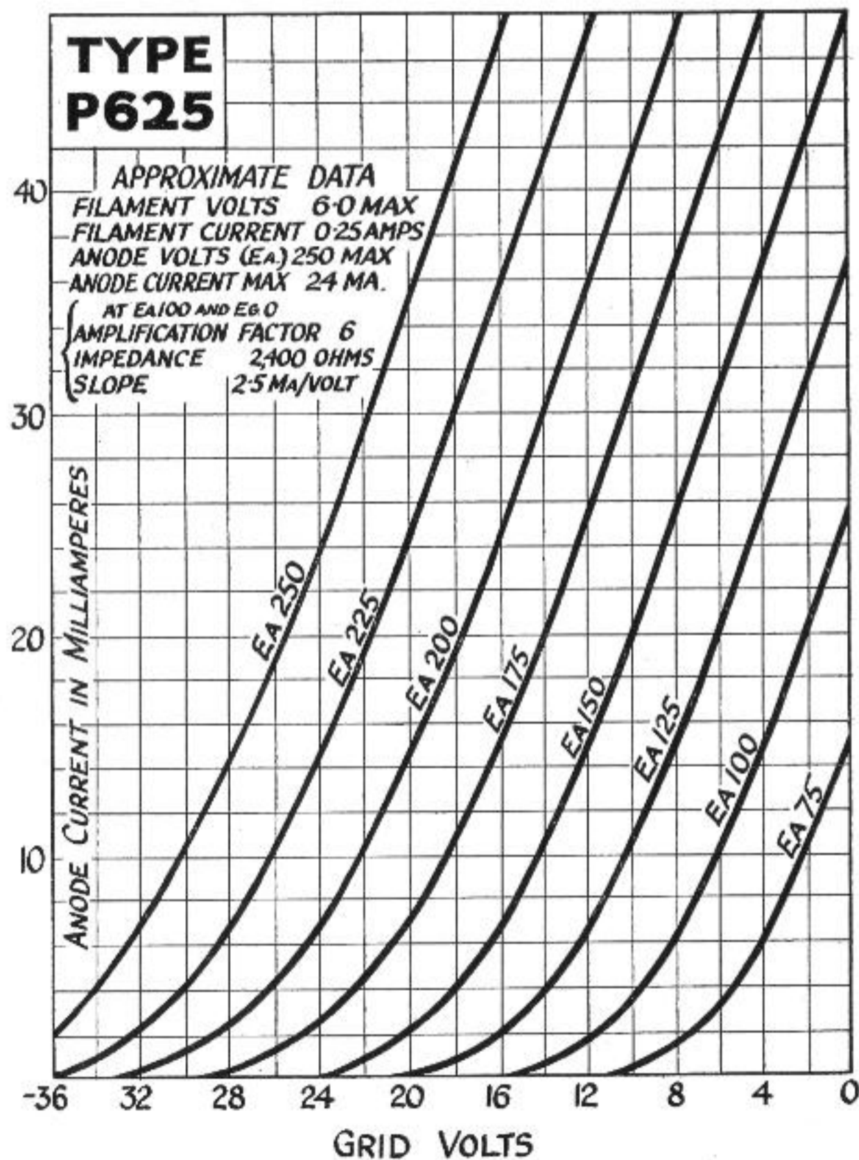
Characteristic Curve of Average P 625 Valve.
